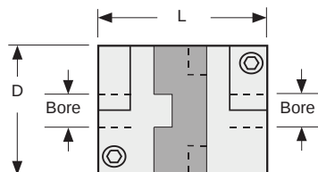
H Type - 3 Member Clamp Style Design
