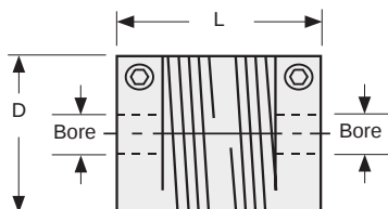
C Type - Aluminum Helical-Cut Clamp Style Design
